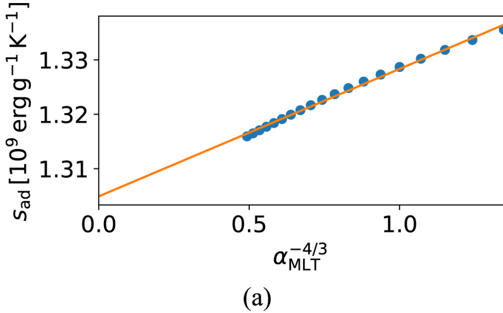
Figure 5. from The Radius and Entropy of a Magnetized, Rotating, Fully Convective Star: Analysis with Depth-dependent Mixing Length Theories null 2018 APJ 856 132 doi:10.3847/1538-4357/aab3da https://dx.doi.org/10.3847/1538-4357/aab3da © 2018. The American Astronomical Society. All rights reserved.
