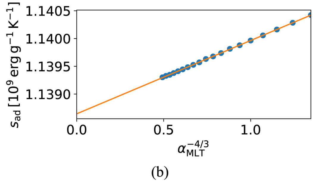
Figure 5. from The Radius and Entropy of a Magnetized, Rotating, Fully Convective Star: Analysis with Depth-dependent Mixing Length Theories null 2018 APJ 856 132 doi:10.3847/1538-4357/aab3da https://dx.doi.org/10.3847/1538-4357/aab3da © 2018. The American Astronomical Society. All rights reserved.
