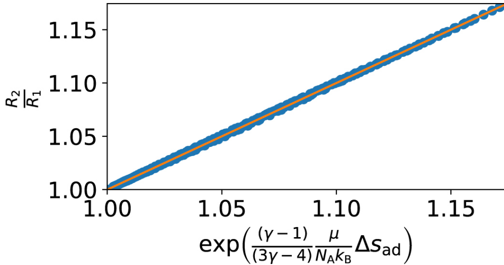
Figure 4. from The Radius and Entropy of a Magnetized, Rotating, Fully Convective Star: Analysis with Depth-dependent Mixing Length Theories null 2018 APJ 856 132 doi:10.3847/1538-4357/aab3da https://dx.doi.org/10.3847/1538-4357/aab3da © 2018. The American Astronomical Society. All rights reserved.
