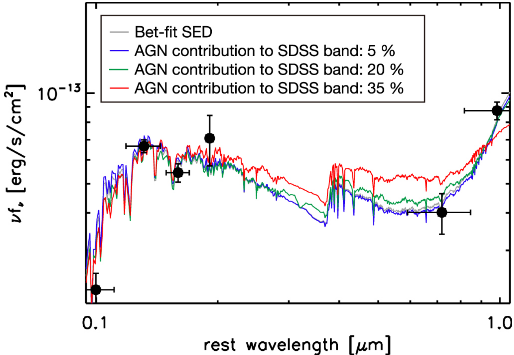
Figure 6. from Discovery of an Extremely Luminous Dust-obscured Galaxy Observed with SDSS, WISE, JCMT, and SMA null 2018 APJ 857 31 doi:10.3847/1538-4357/aab3cf https://dx.doi.org/10.3847/1538-4357/aab3cf © 2018. The American Astronomical Society. All rights reserved.
