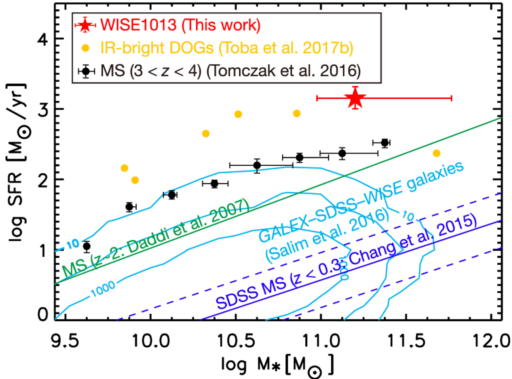
Figure 5. from Discovery of an Extremely Luminous Dust-obscured Galaxy Observed with SDSS, WISE, JCMT, and SMA null 2018 APJ 857 31 doi:10.3847/1538-4357/aab3cf https://dx.doi.org/10.3847/1538-4357/aab3cf © 2018. The American Astronomical Society. All rights reserved.
