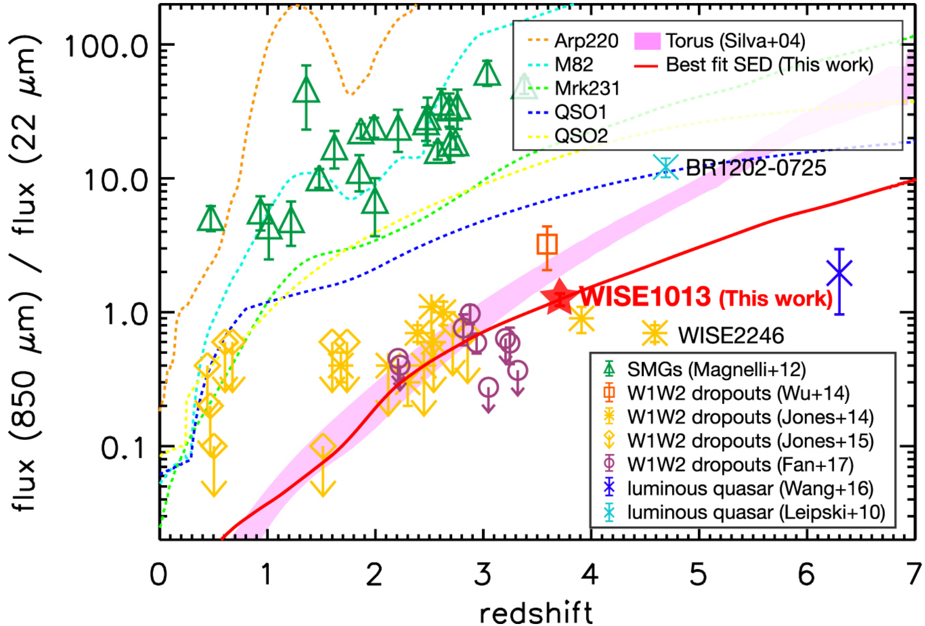
Figure 4. from Discovery of an Extremely Luminous Dust-obscured Galaxy Observed with SDSS, WISE, JCMT, and SMA null 2018 APJ 857 31 doi:10.3847/1538-4357/aab3cf https://dx.doi.org/10.3847/1538-4357/aab3cf © 2018. The American Astronomical Society. All rights reserved.
