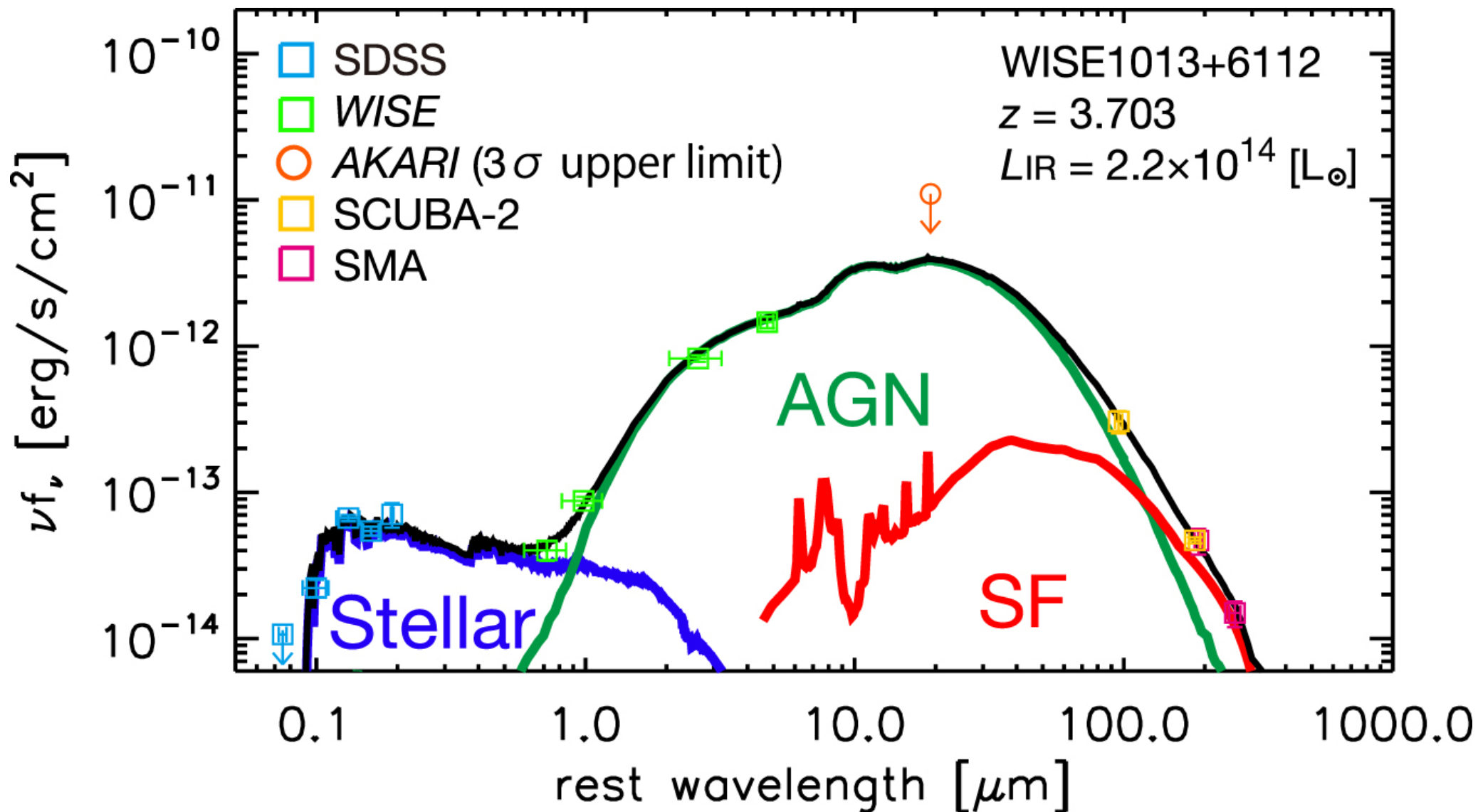
Figure 2. from Discovery of an Extremely Luminous Dust-obscured Galaxy Observed with SDSS, WISE, JCMT, and SMA null 2018 APJ 857 31 doi:10.3847/1538-4357/aab3cf https://dx.doi.org/10.3847/1538-4357/aab3cf © 2018. The American Astronomical Society. All rights reserved.
