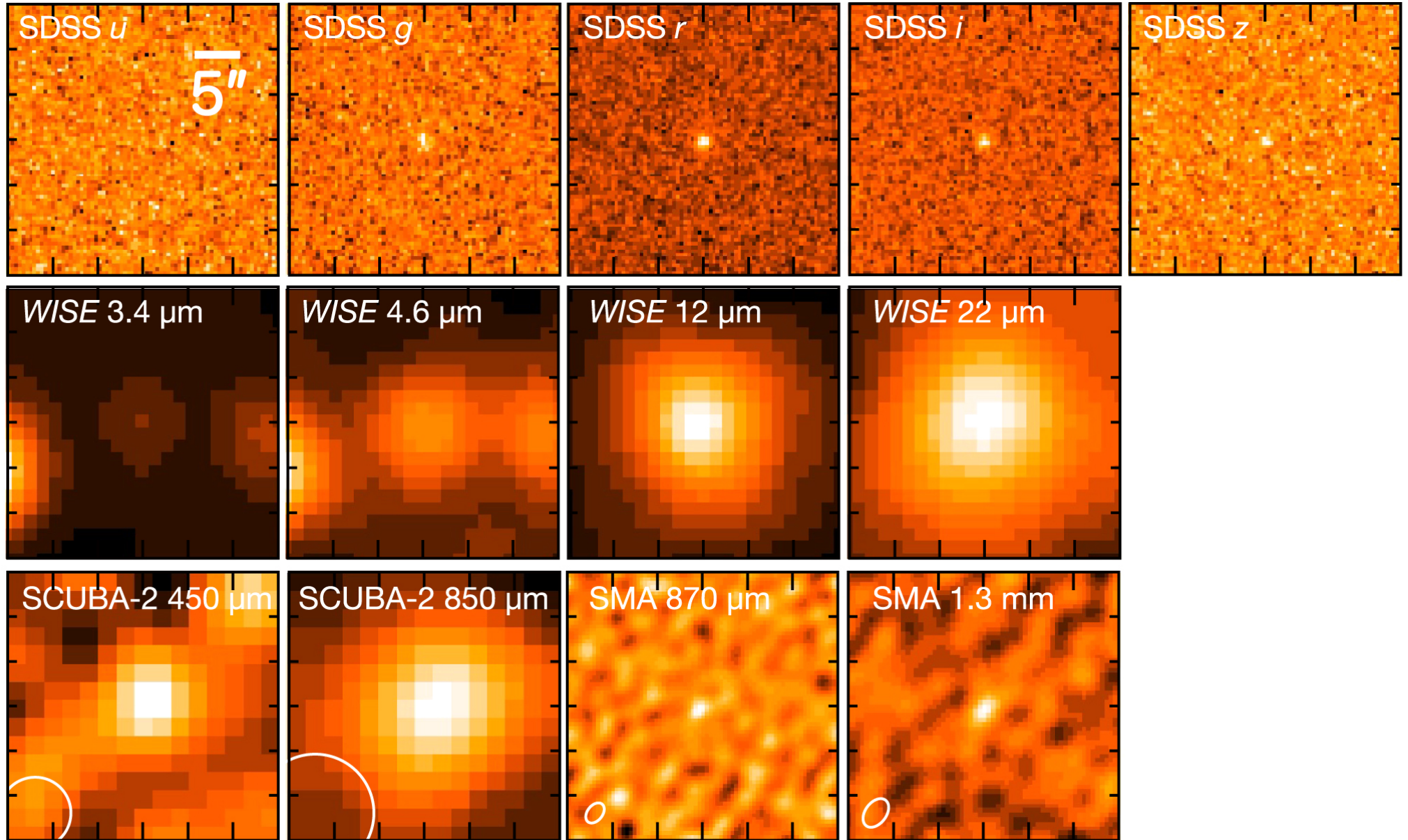
Figure 1. from Discovery of an Extremely Luminous Dust-obscured Galaxy Observed with SDSS, WISE, JCMT, and SMA null 2018 APJ 857 31 doi:10.3847/1538-4357/aab3cf https://dx.doi.org/10.3847/1538-4357/aab3cf © 2018. The American Astronomical Society. All rights reserved.
