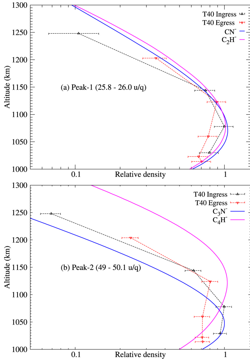
Figure 9. from A Model for Negative Ion Chemistry in Titan's Ionosphere null 2018 APJ 856 168 doi:10.3847/1538-4357/aab1f5 https://dx.doi.org/10.3847/1538-4357/aab1f5
