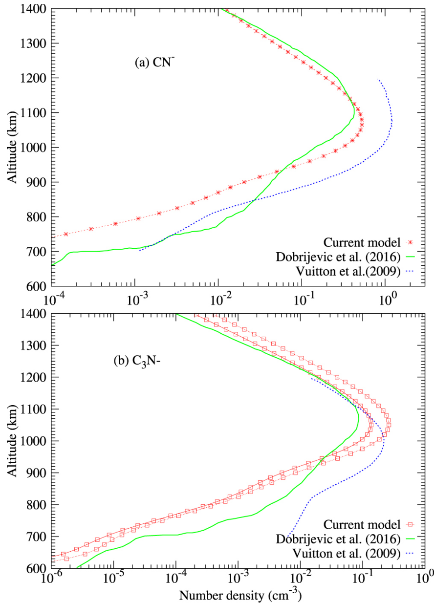
Figure 4. from A Model for Negative Ion Chemistry in Titan's Ionosphere null 2018 APJ 856 168 doi:10.3847/1538-4357/aab1f5 https://dx.doi.org/10.3847/1538-4357/aab1f5
