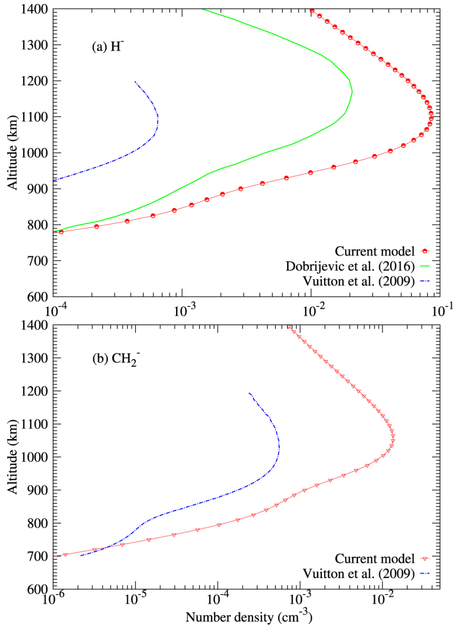
Figure 3. from A Model for Negative Ion Chemistry in Titan's Ionosphere null 2018 APJ 856 168 doi:10.3847/1538-4357/aab1f5 https://dx.doi.org/10.3847/1538-4357/aab1f5
