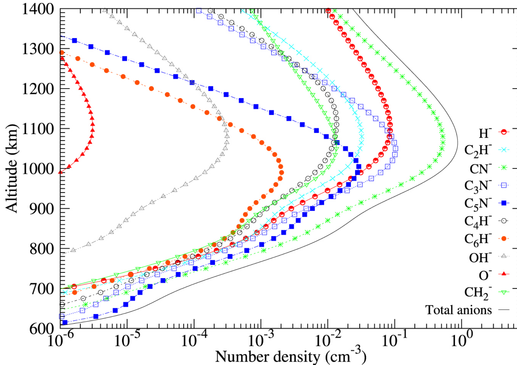
Figure 2. from A Model for Negative Ion Chemistry in Titan's Ionosphere null 2018 APJ 856 168 doi:10.3847/1538-4357/aab1f5 https://dx.doi.org/10.3847/1538-4357/aab1f5 © 2018. The American Astronomical Society. All rights reserved.
