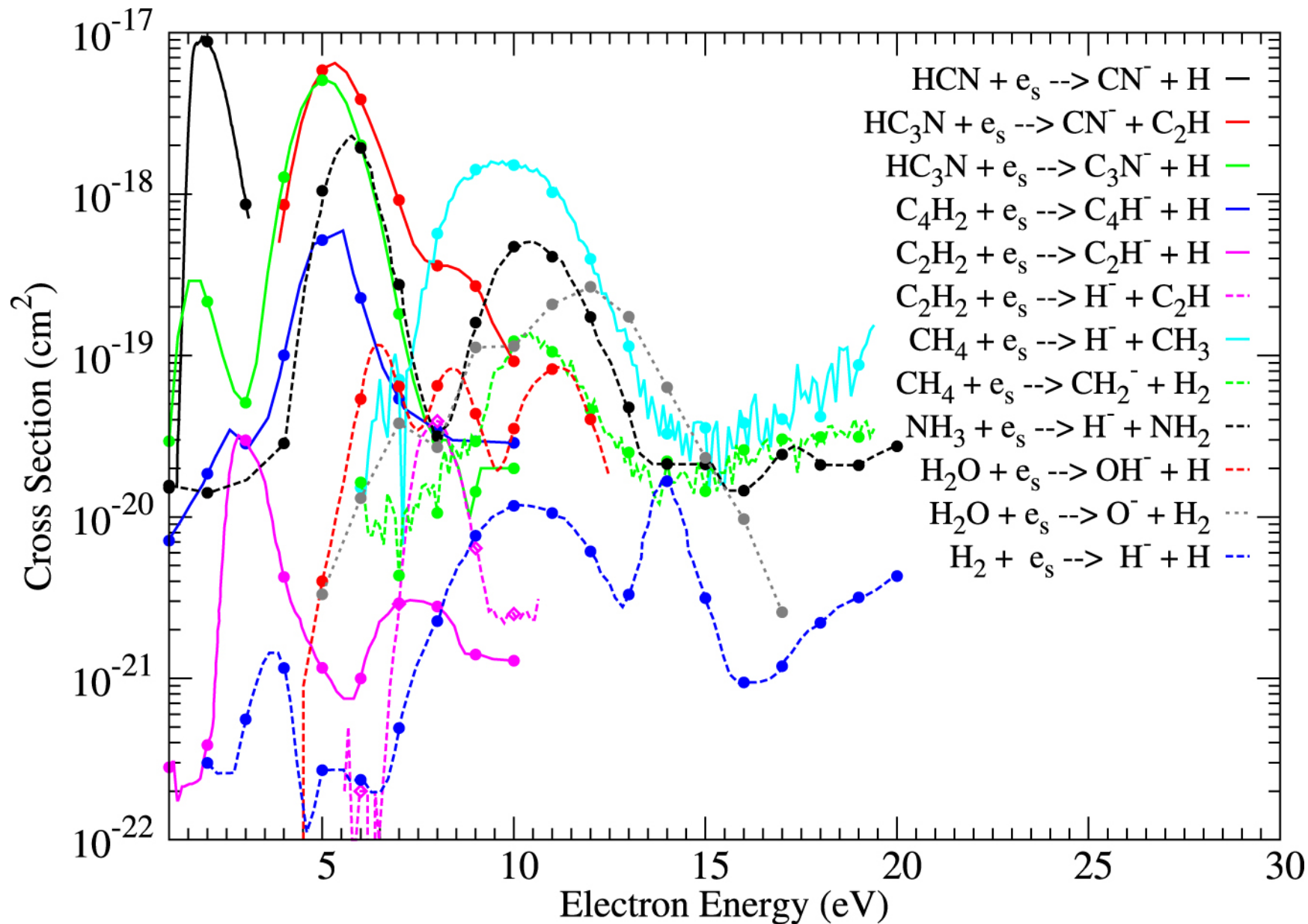
Figure 1. from A Model for Negative Ion Chemistry in Titan's Ionosphere null 2018 APJ 856 168 doi:10.3847/1538-4357/aab1f5 https://dx.doi.org/10.3847/1538-4357/aab1f5 © 2018. The American Astronomical Society. All rights reserved.
