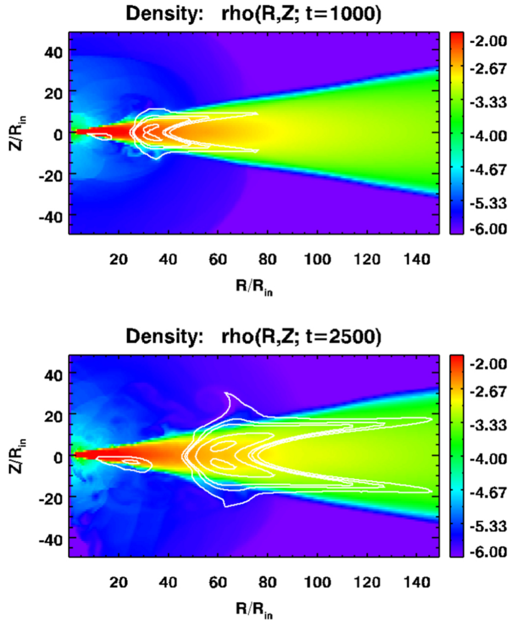
Figure 8. from Bipolar Jets Launched by a Mean-field Accretion Disk Dynamo null 2018 APJ 855 130 doi:10.3847/1538-4357/aab14c https://dx.doi.org/10.3847/1538-4357/aab14c © 2018. The American Astronomical Society. All rights reserved.
