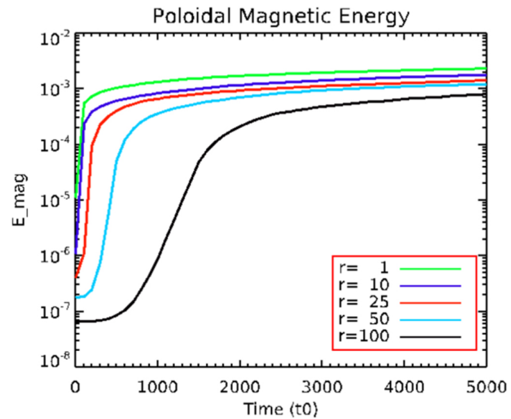
Figure 7. from Bipolar Jets Launched by a Mean-field Accretion Disk Dynamo null 2018 APJ 855 130 doi:10.3847/1538-4357/aab14c https://dx.doi.org/10.3847/1538-4357/aab14c © 2018. The American Astronomical Society. All rights reserved.
