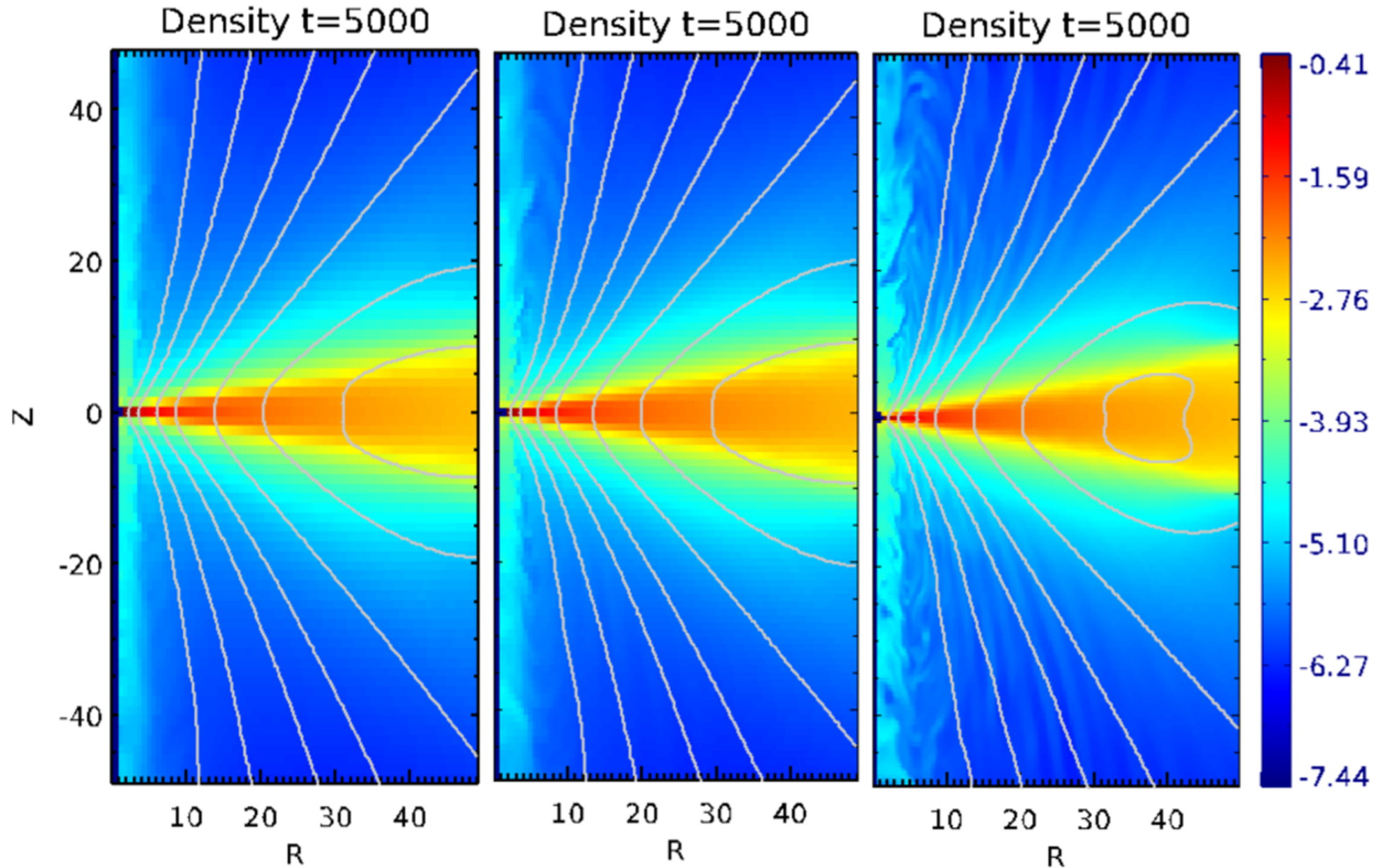
Figure 23. from Bipolar Jets Launched by a Mean-field Accretion Disk Dynamo null 2018 APJ 855 130 doi:10.3847/1538-4357/aab14c https://dx.doi.org/10.3847/1538-4357/aab14c © 2018. The American Astronomical Society. All rights reserved.
