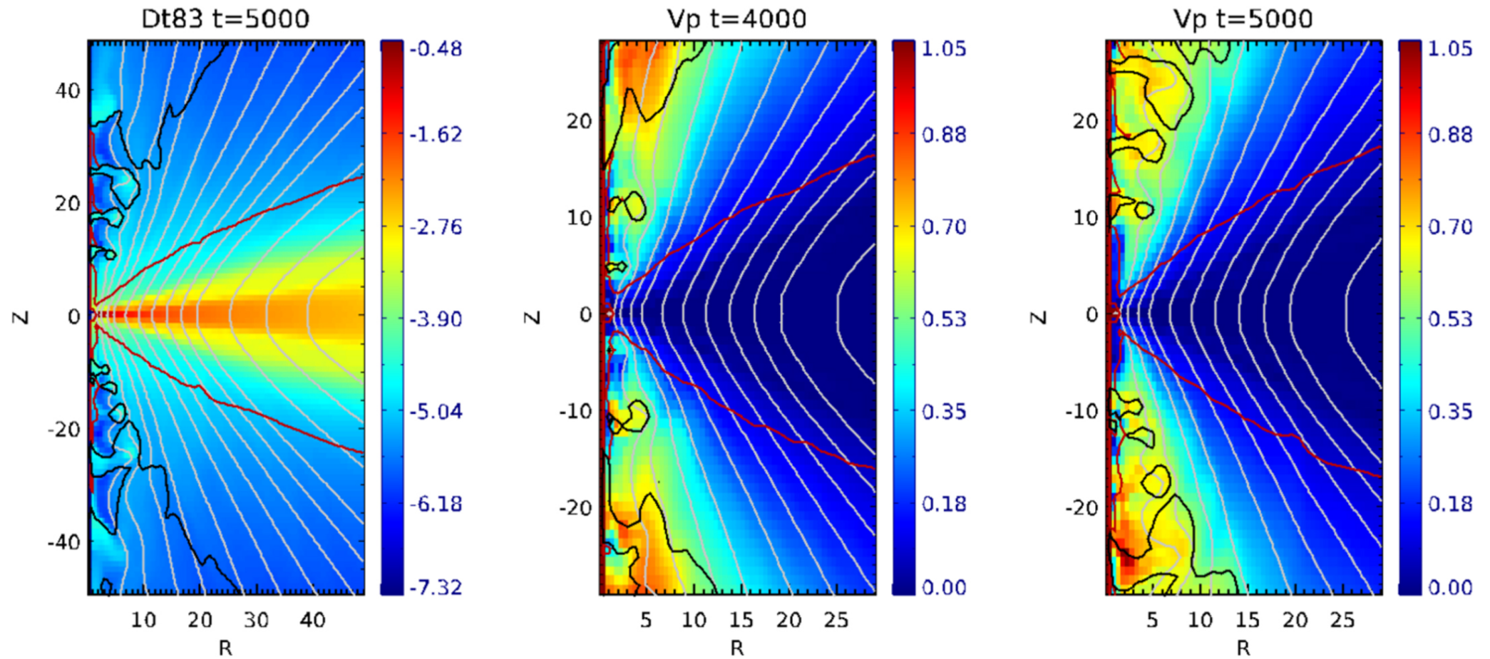
Figure 17. from Bipolar Jets Launched by a Mean-field Accretion Disk Dynamo null 2018 APJ 855 130 doi:10.3847/1538-4357/aab14c https://dx.doi.org/10.3847/1538-4357/aab14c © 2018. The American Astronomical Society. All rights reserved.
