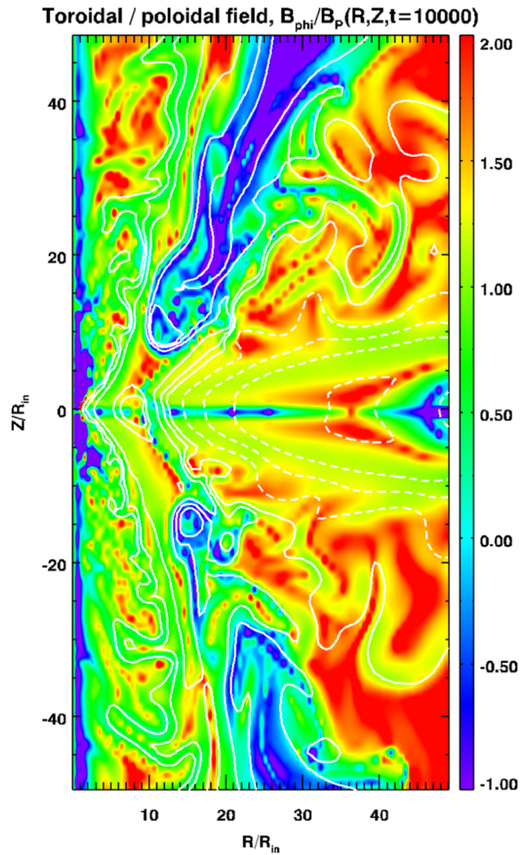
Figure 16. from Bipolar Jets Launched by a Mean-field Accretion Disk Dynamo null 2018 APJ 855 130 doi:10.3847/1538-4357/aab14c https://dx.doi.org/10.3847/1538-4357/aab14c © 2018. The American Astronomical Society. All rights reserved.
