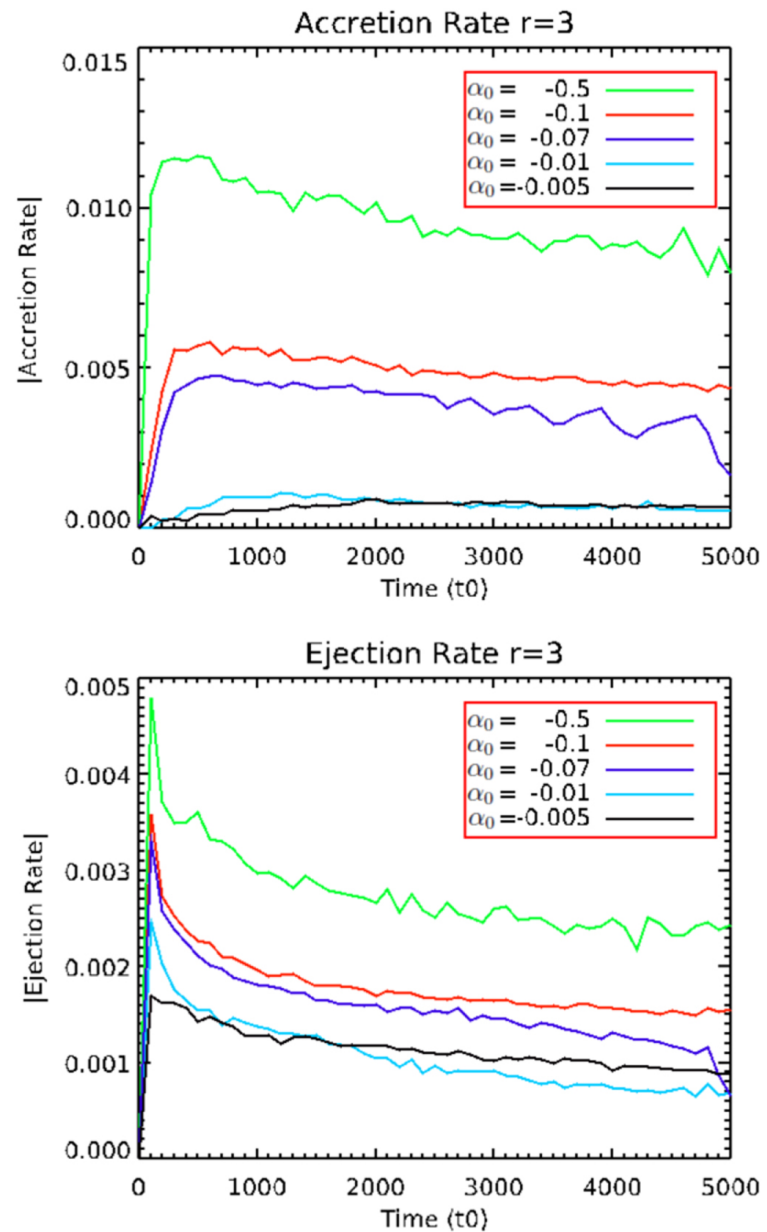
Figure 12. from Bipolar Jets Launched by a Mean-field Accretion Disk Dynamo null 2018 APJ 855 130 doi:10.3847/1538-4357/aab14c https://dx.doi.org/10.3847/1538-4357/aab14c © 2018. The American Astronomical Society. All rights reserved.
