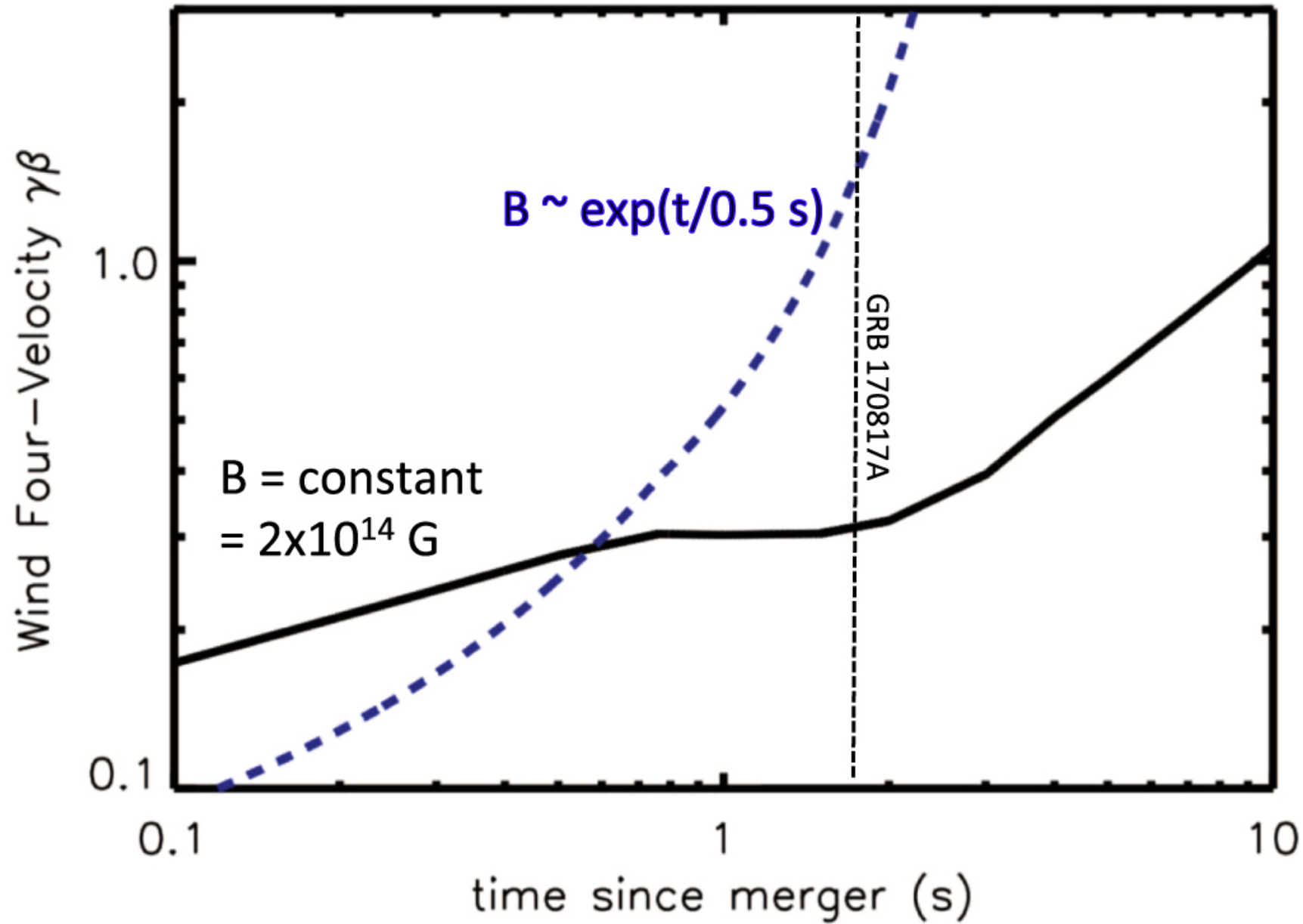
Figure 4. from A Magnetar Origin for the Kilonova Ejecta in GW170817 null 2018 APJ 856 101 doi:10.3847/1538-4357/aab095 https://dx.doi.org/10.3847/1538-4357/aab095 © 2018. The American Astronomical Society. All rights reserved.
