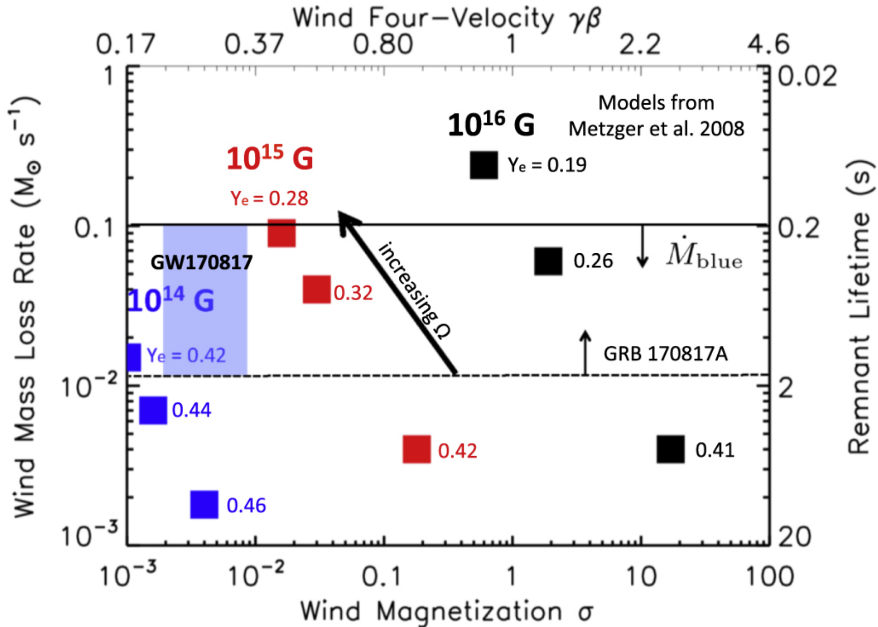
Figure 2. from A Magnetar Origin for the Kilonova Ejecta in GW170817 null 2018 APJ 856 101 doi:10.3847/1538-4357/aab095 https://dx.doi.org/10.3847/1538-4357/aab095 © 2018. The American Astronomical Society. All rights reserved.
