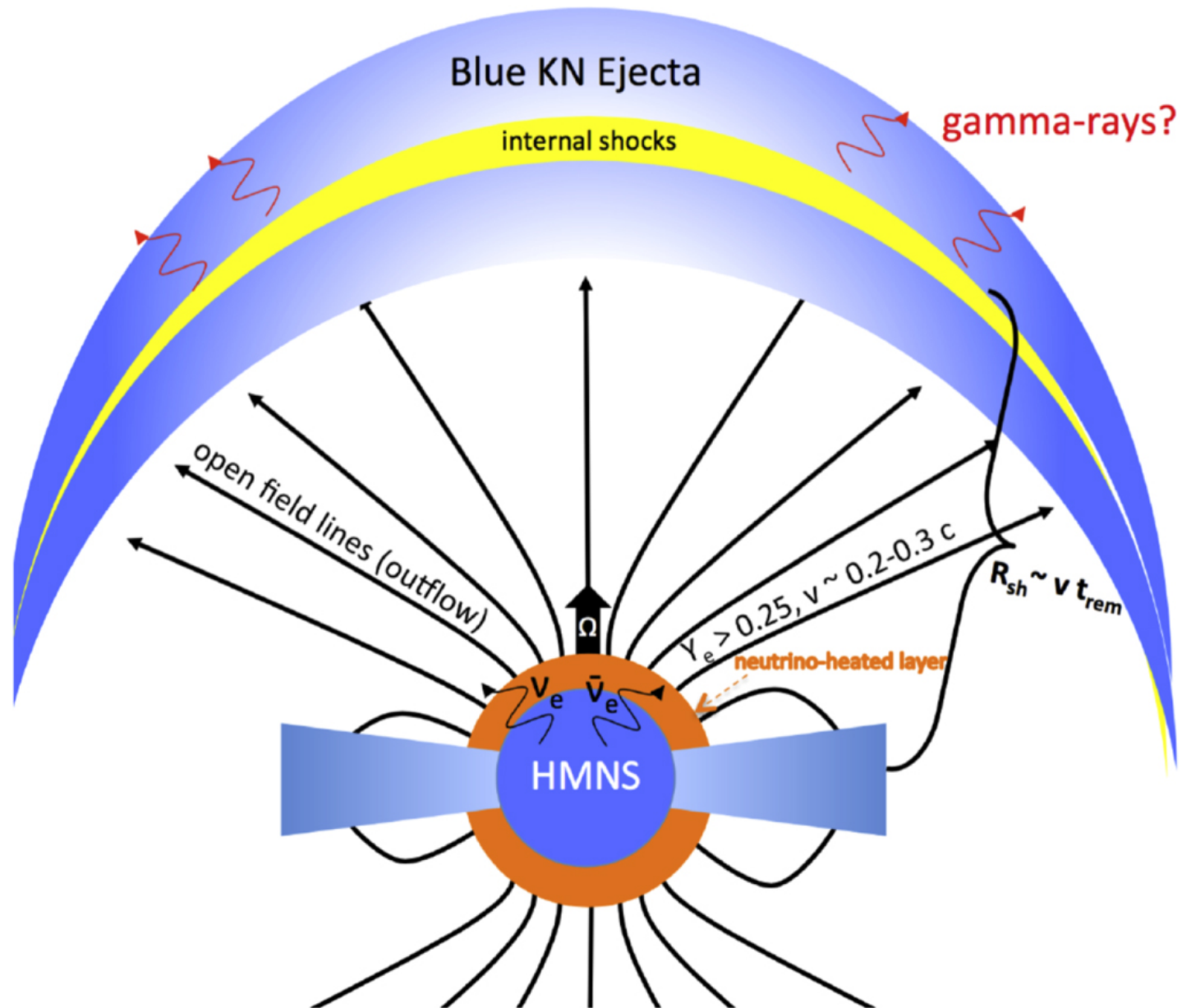
Figure 1. from A Magnetar Origin for the Kilonova Ejecta in GW170817 null 2018 APJ 856 101 doi:10.3847/1538-4357/aab095 https://dx.doi.org/10.3847/1538-4357/aab095 © 2018. The American Astronomical Society. All rights reserved.
