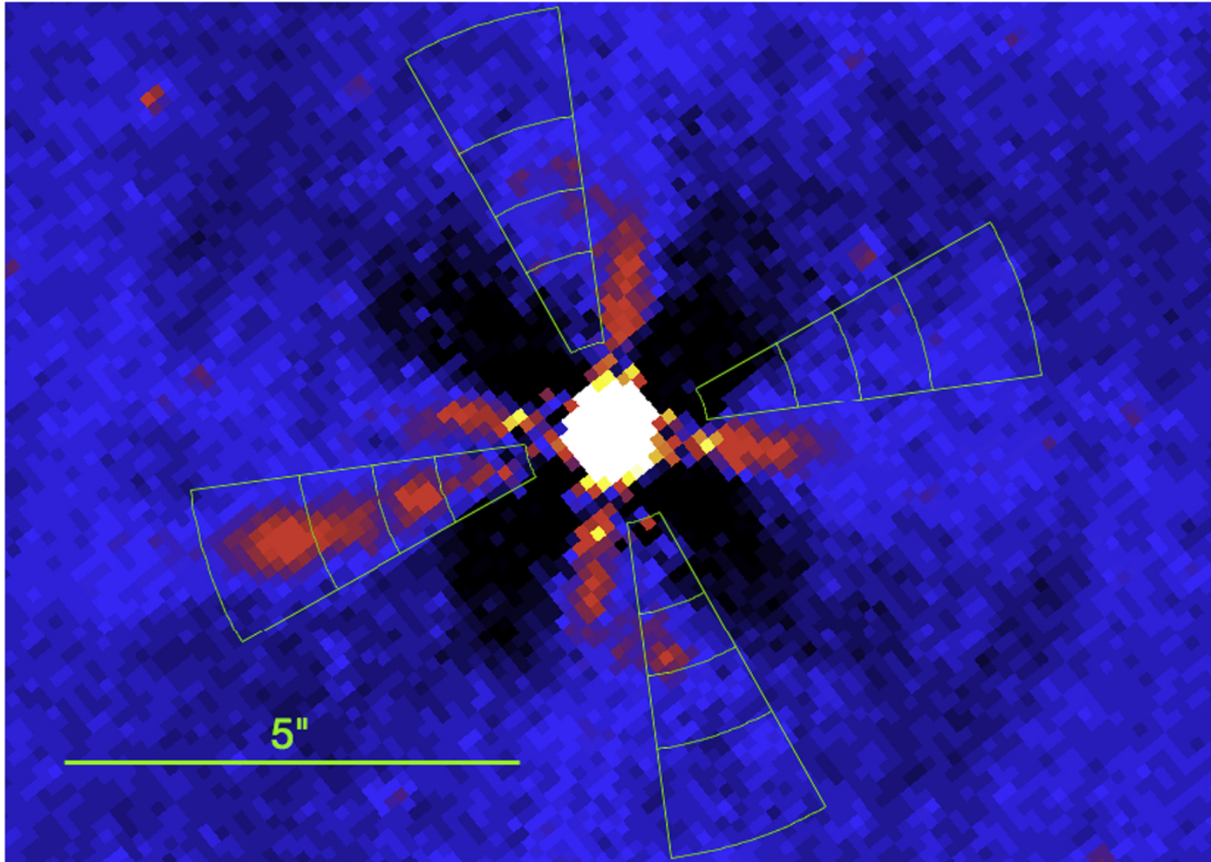
Figure 8. from An X-Ray Imaging Survey of Quasar Jets: The Complete Survey null 2018 APJ 856 66 doi:10.3847/1538-4357/aaaf66 https://dx.doi.org/10.3847/1538-4357/aaaf66 © 2018. The American Astronomical Society.
