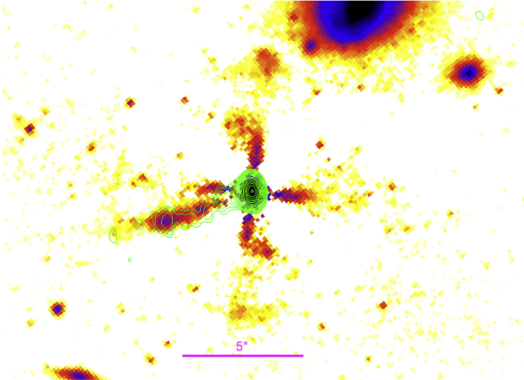
Figure 7. from An X-Ray Imaging Survey of Quasar Jets: The Complete Survey null 2018 APJ 856 66 doi:10.3847/1538-4357/aaaf66 https://dx.doi.org/10.3847/1538-4357/aaaf66 © 2018. The American Astronomical Society.
