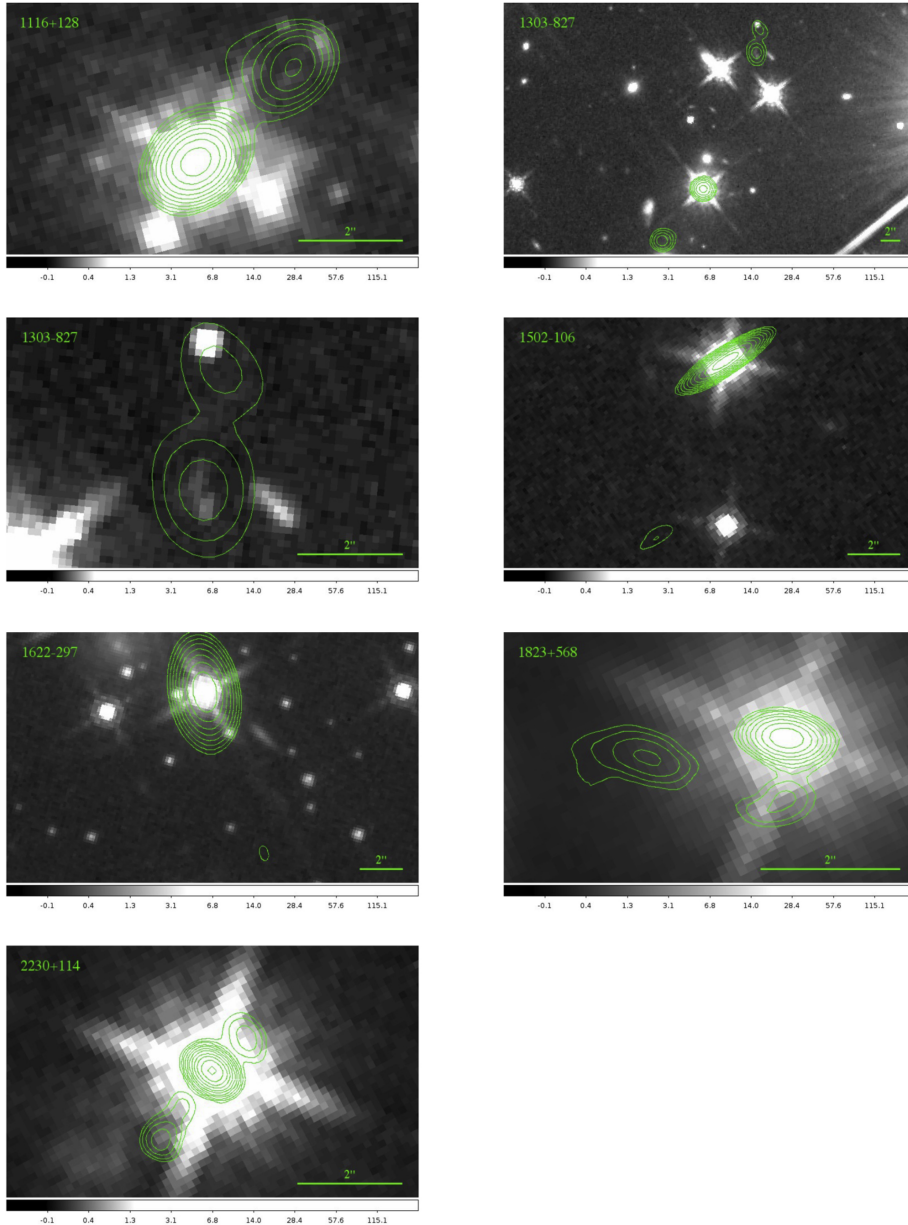
Figure 6. from An X-Ray Imaging Survey of Quasar Jets: The Complete Survey null 2018 APJ 856 66 doi:10.3847/1538-4357/aaaf66 https://dx.doi.org/10.3847/1538-4357/aaaf66 © 2018. The American Astronomical Society.
