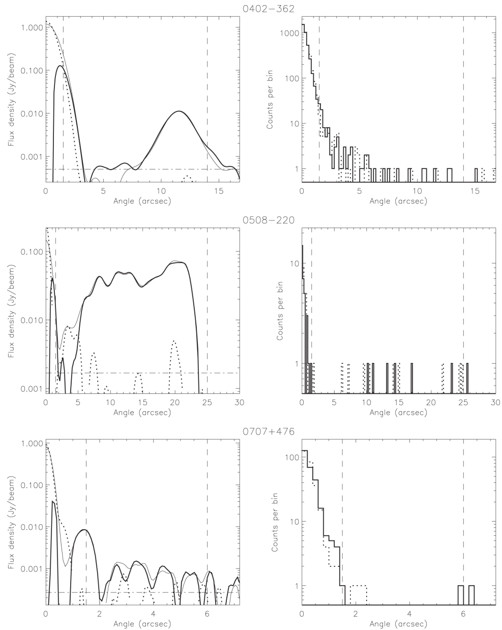
Figure 5. from An X-Ray Imaging Survey of Quasar Jets: The Complete Survey null 2018 APJ 856 66 doi:10.3847/1538-4357/aaaf66 https://dx.doi.org/10.3847/1538-4357/aaaf66 © 2018. The American Astronomical Society.
