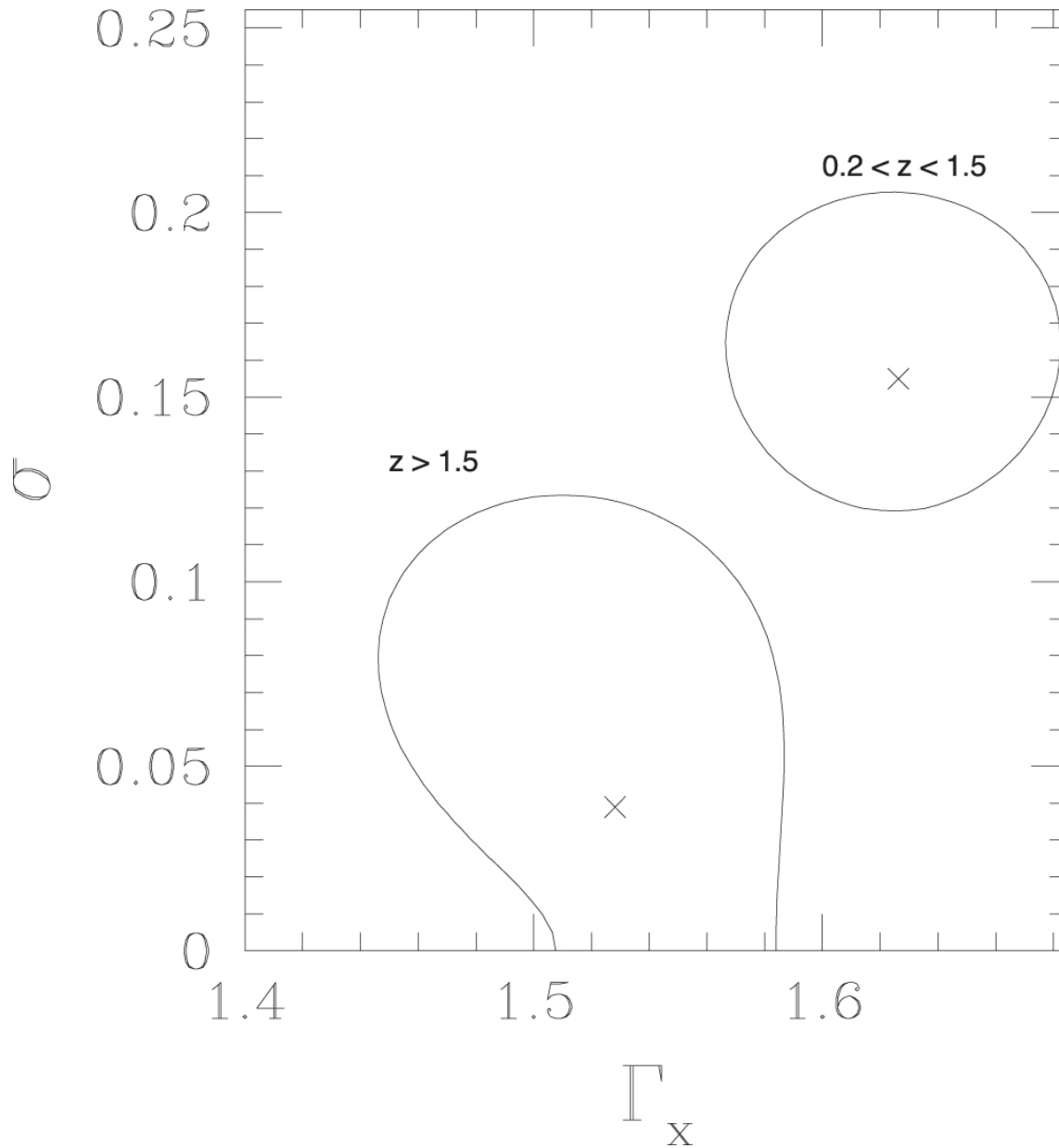
Figure 3. from An X-Ray Imaging Survey of Quasar Jets: The Complete Survey null 2018 APJ 856 66 doi:10.3847/1538-4357/aaaf66 https://dx.doi.org/10.3847/1538-4357/aaaf66 © 2018. The American Astronomical Society.
