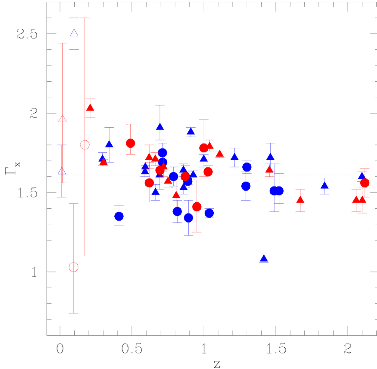
Figure 2. from An X-Ray Imaging Survey of Quasar Jets: The Complete Survey null 2018 APJ 856 66 doi:10.3847/1538-4357/aaaf66 https://dx.doi.org/10.3847/1538-4357/aaaf66 © 2018. The American Astronomical Society.
