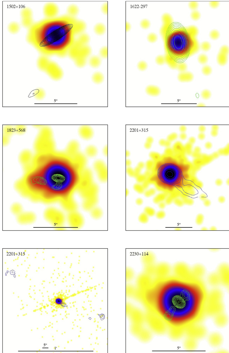
Figure 1. from An X-Ray Imaging Survey of Quasar Jets: The Complete Survey null 2018 APJ 856 66 doi:10.3847/1538-4357/aaaf66 https://dx.doi.org/10.3847/1538-4357/aaaf66 © 2018. The American Astronomical Society.
