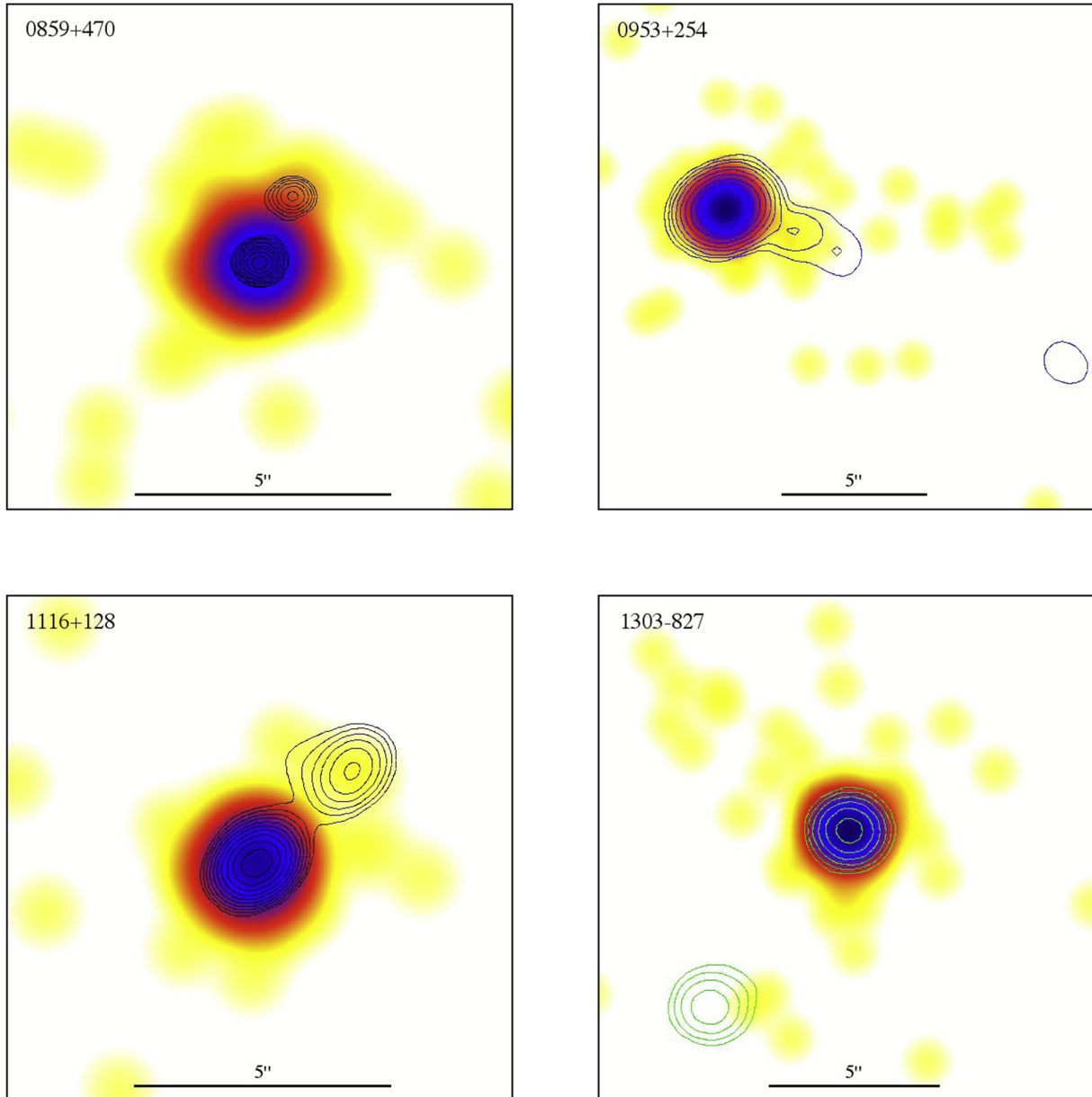
Figure 1. from An X-Ray Imaging Survey of Quasar Jets: The Complete Survey null 2018 APJ 856 66 doi:10.3847/1538-4357/aaaf66 https://dx.doi.org/10.3847/1538-4357/aaaf66 © 2018. The American Astronomical Society.
