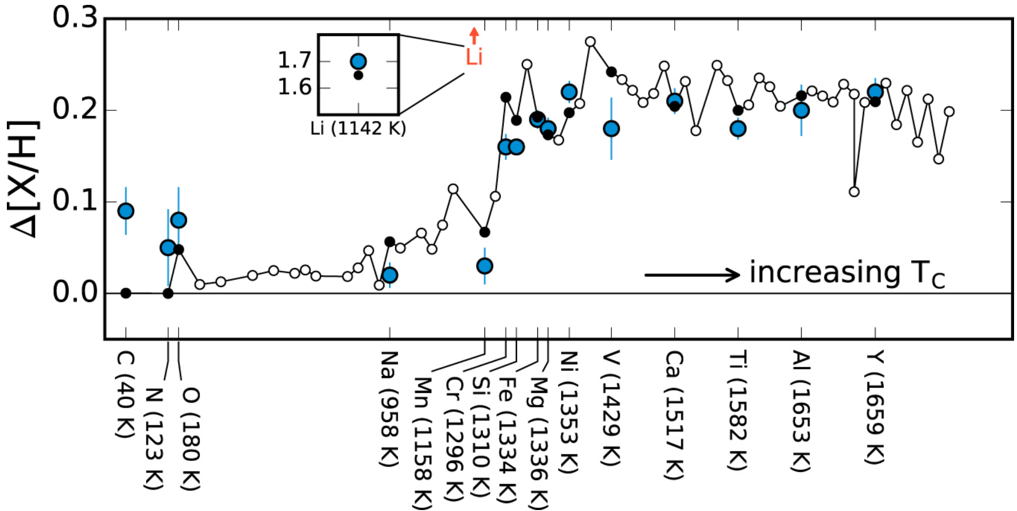
Figure 9. from Kronos and Krios: Evidence for Accretion of a Massive, Rocky Planetary System in a Comoving Pair of Solar-type Stars null 2018 APJ 854 138 doi:10.3847/1538-4357/aaab4d https://dx.doi.org/10.3847/1538-4357/aaab4d © 2018. The American Astronomical Society. All rights reserved.
