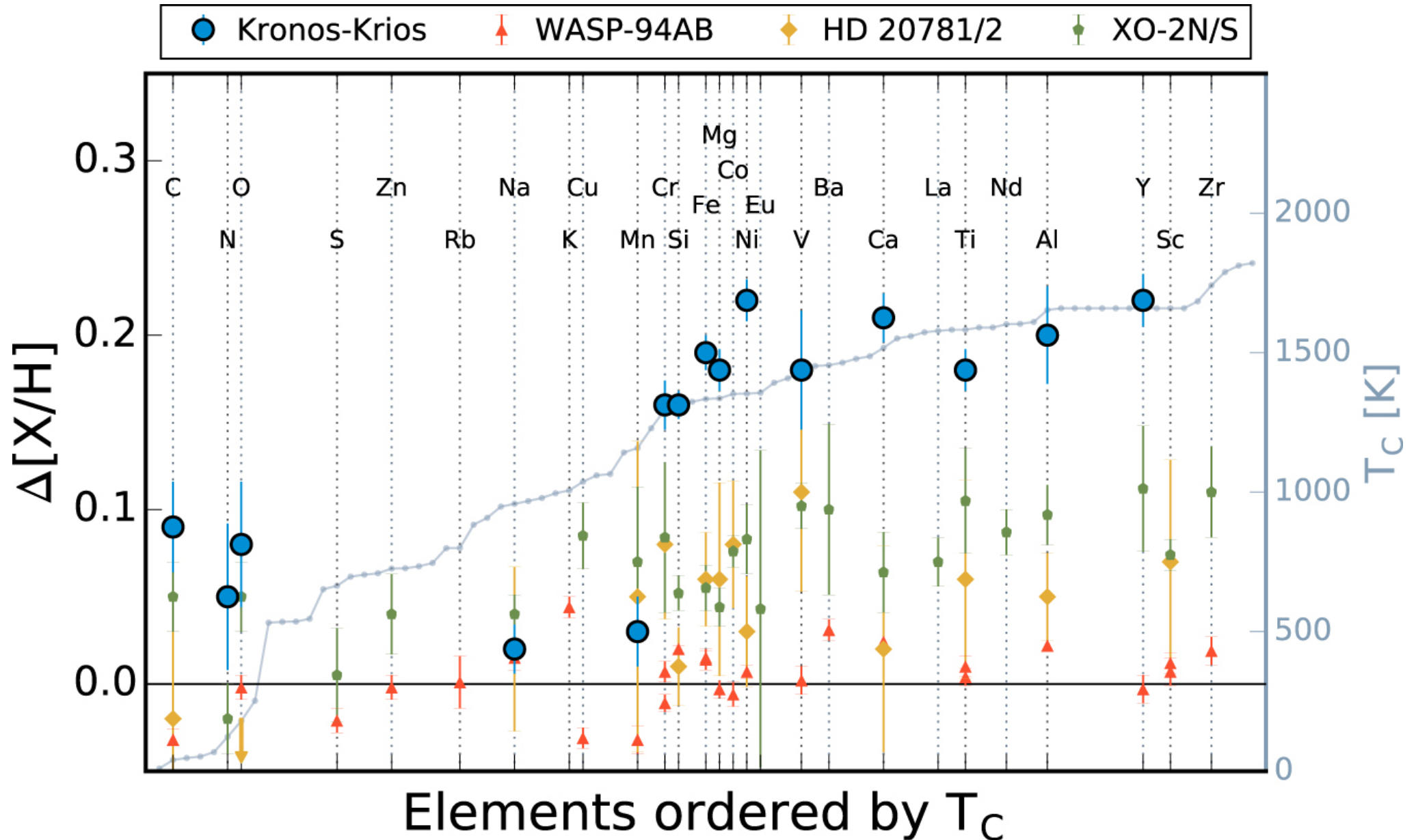
Figure 8. from Kronos and Krios: Evidence for Accretion of a Massive, Rocky Planetary System in a Comoving Pair of Solar-type Stars null 2018 APJ 854 138 doi:10.3847/1538-4357/aaab4d https://dx.doi.org/10.3847/1538-4357/aaab4d © 2018. The American Astronomical Society. All rights reserved.
