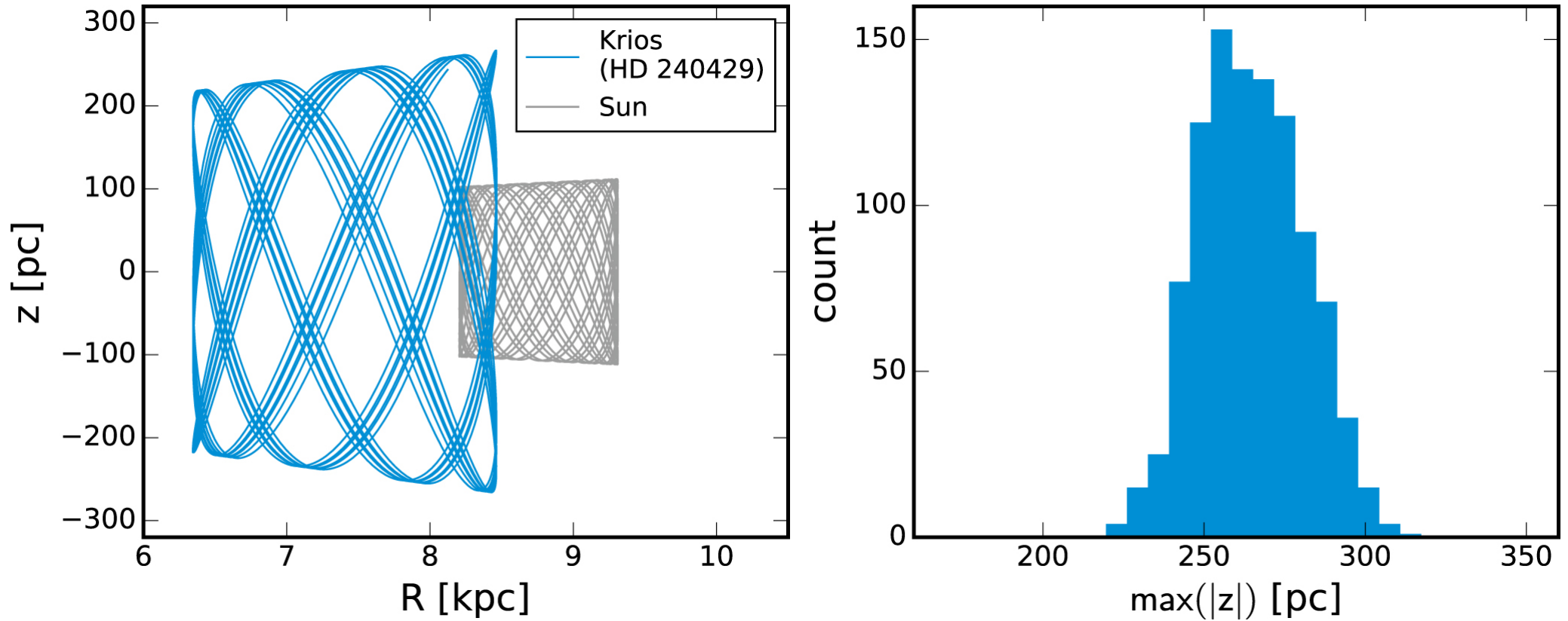
Figure 7. from Kronos and Krios: Evidence for Accretion of a Massive, Rocky Planetary System in a Comoving Pair of Solar-type Stars null 2018 APJ 854 138 doi:10.3847/1538-4357/aaab4d https://dx.doi.org/10.3847/1538-4357/aaab4d © 2018. The American Astronomical Society. All rights reserved.
