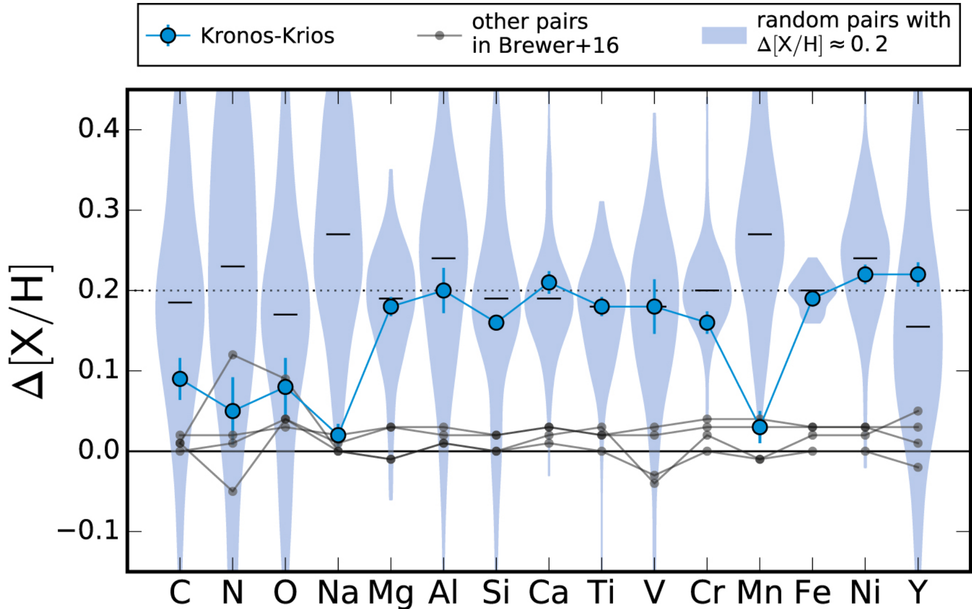
Figure 6. from Kronos and Krios: Evidence for Accretion of a Massive, Rocky Planetary System in a Comoving Pair of Solar-type Stars null 2018 APJ 854 138 doi:10.3847/1538-4357/aaab4d https://dx.doi.org/10.3847/1538-4357/aaab4d © 2018. The American Astronomical Society. All rights reserved.
