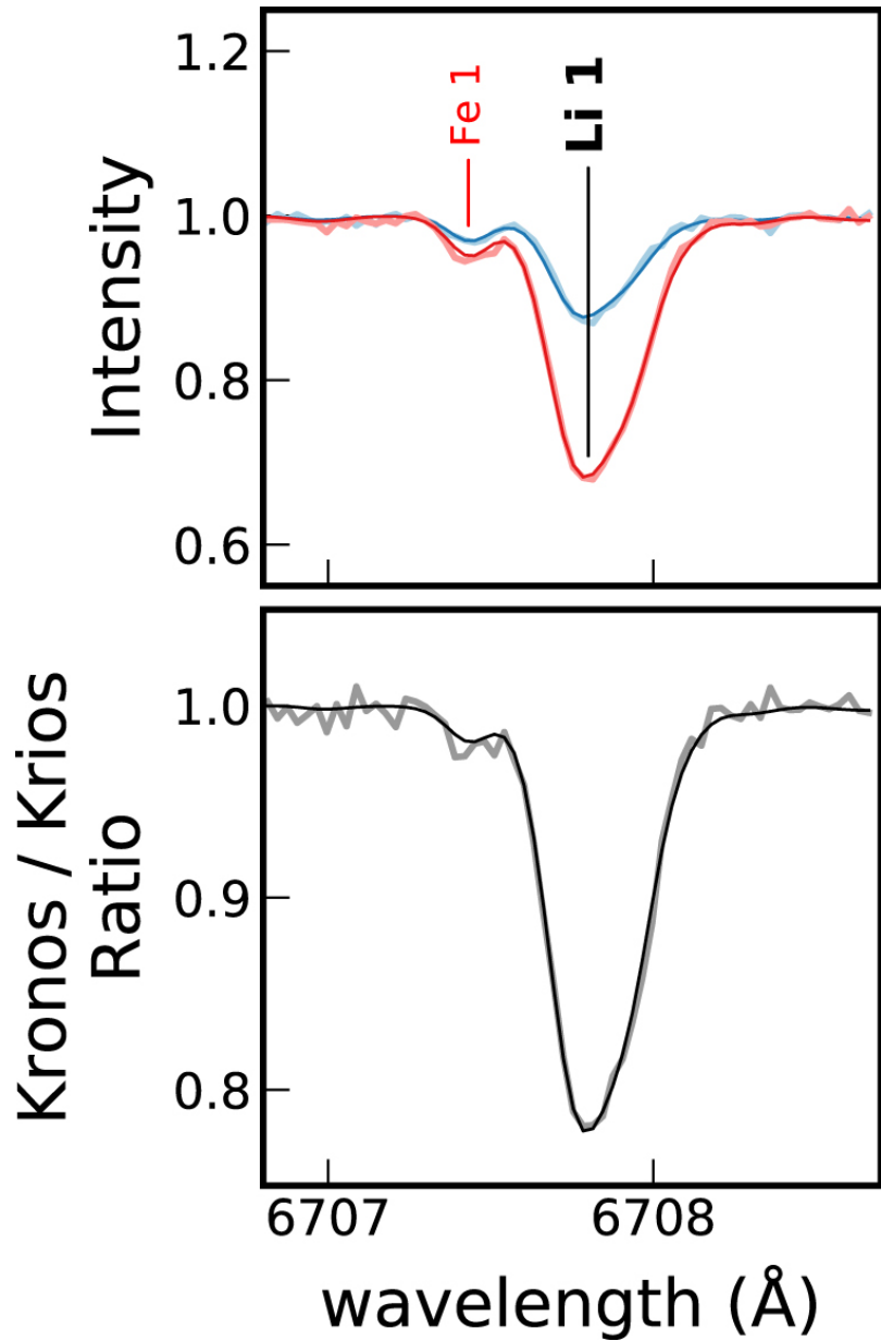
Figure 5. from Kronos and Krios: Evidence for Accretion of a Massive, Rocky Planetary System in a Comoving Pair of Solar-type Stars null 2018 APJ 854 138 doi:10.3847/1538-4357/aaab4d https://dx.doi.org/10.3847/1538-4357/aaab4d © 2018. The American Astronomical Society. All rights reserved.
