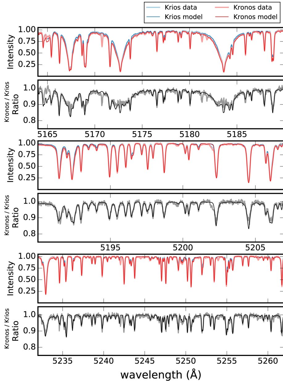
Figure 3. from Kronos and Krios: Evidence for Accretion of a Massive, Rocky Planetary System in a Comoving Pair of Solar-type Stars null 2018 APJ 854 138 doi:10.3847/1538-4357/aaab4d https://dx.doi.org/10.3847/1538-4357/aaab4d © 2018. The American Astronomical Society. All rights reserved.
