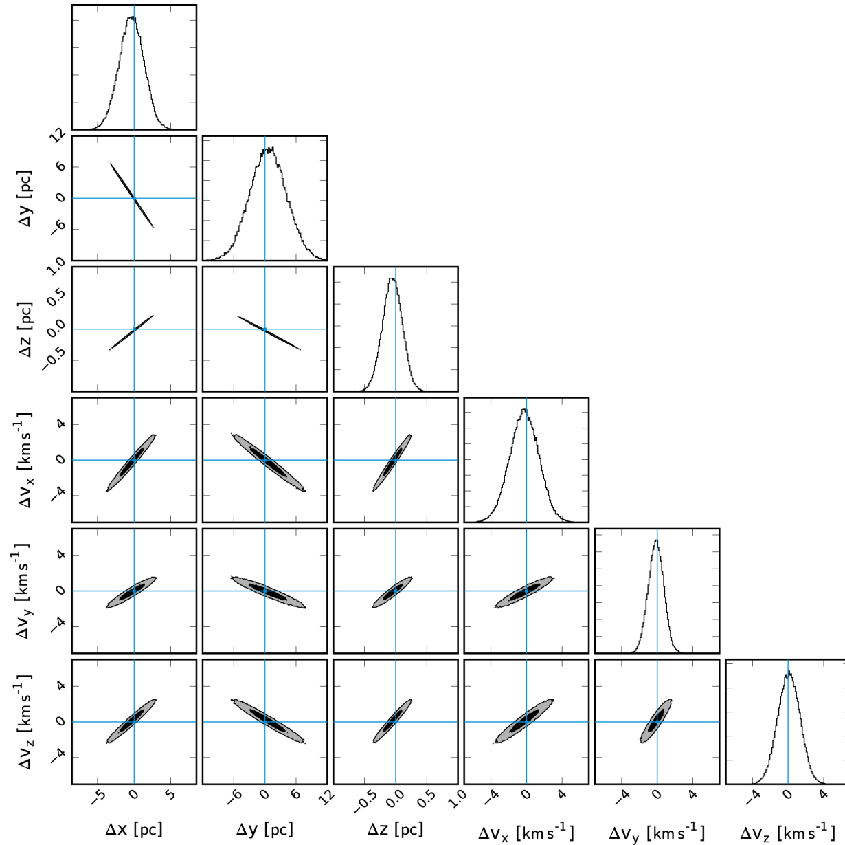
Figure 1. from Kronos and Krios: Evidence for Accretion of a Massive, Rocky Planetary System in a Comoving Pair of Solar-type Stars null 2018 APJ 854 138 doi:10.3847/1538-4357/aaab4d https://dx.doi.org/10.3847/1538-4357/aaab4d © 2018. The American Astronomical Society. All rights reserved.
