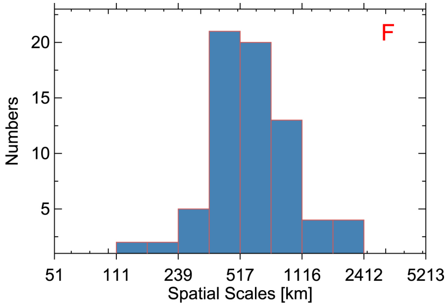
Figure 5. from Fine Structures of Solar Radio Type III Bursts and Their Possible Relationship with Coronal Density Turbulence null 2018 APJ 856 73 doi:10.3847/1538-4357/aaa9bf https://dx.doi.org/10.3847/1538-4357/aaa9bf © 2018. The American Astronomical Society.
