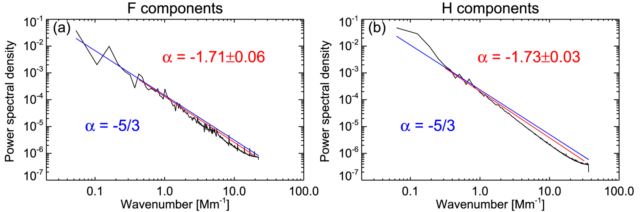
Figure 4. from Fine Structures of Solar Radio Type III Bursts and Their Possible Relationship with Coronal Density Turbulence null 2018 APJ 856 73 doi:10.3847/1538-4357/aaa9bf https://dx.doi.org/10.3847/1538-4357/aaa9bf © 2018. The American Astronomical Society.
