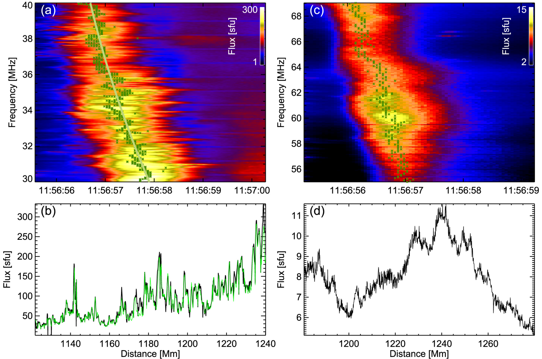
Figure 3. from Fine Structures of Solar Radio Type III Bursts and Their Possible Relationship with Coronal Density Turbulence null 2018 APJ 856 73 doi:10.3847/1538-4357/aaa9bf https://dx.doi.org/10.3847/1538-4357/aaa9bf © 2018. The American Astronomical Society.
