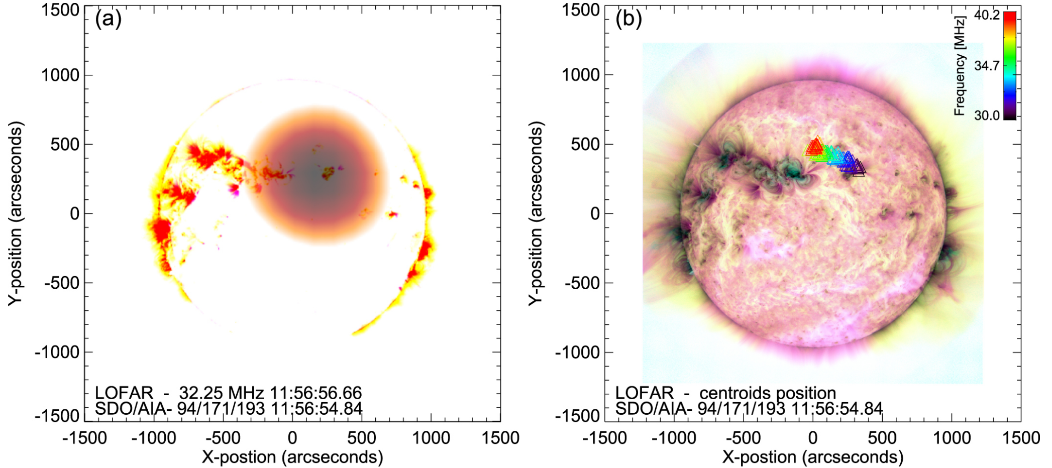
Figure 2. from Fine Structures of Solar Radio Type III Bursts and Their Possible Relationship with Coronal Density Turbulence null 2018 APJ 856 73 doi:10.3847/1538-4357/aaa9bf https://dx.doi.org/10.3847/1538-4357/aaa9bf © 2018. The American Astronomical Society.
