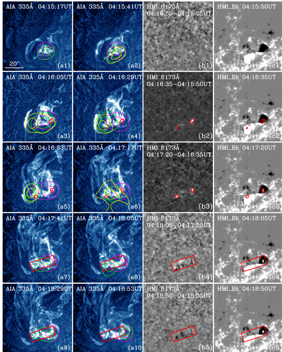
Figure 9. from Observations of a White-light Flare Associated with a Filament Eruption null 2018 APJ 854 64 doi:10.3847/1538-4357/aaa7f1 https://dx.doi.org/10.3847/1538-4357/aaa7f1 © 2018. The American Astronomical Society. All rights reserved.
