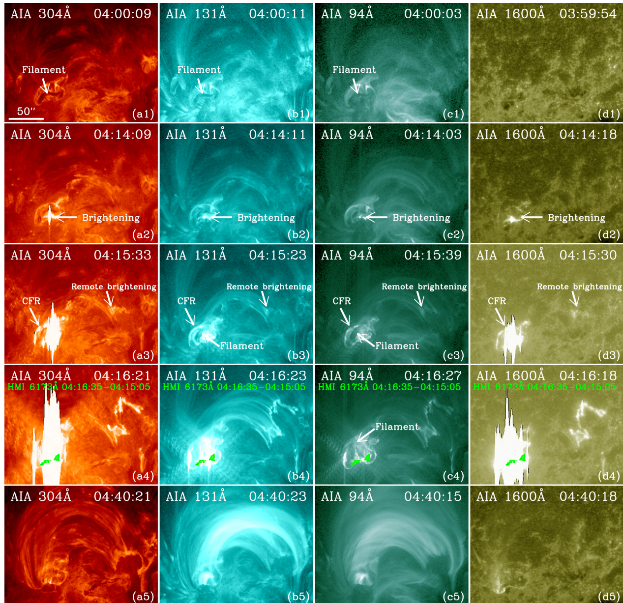
Figure 8. from Observations of a White-light Flare Associated with a Filament Eruption null 2018 APJ 854 64 doi:10.3847/1538-4357/aaa7f1 https://dx.doi.org/10.3847/1538-4357/aaa7f1 © 2018. The American Astronomical Society. All rights reserved.
