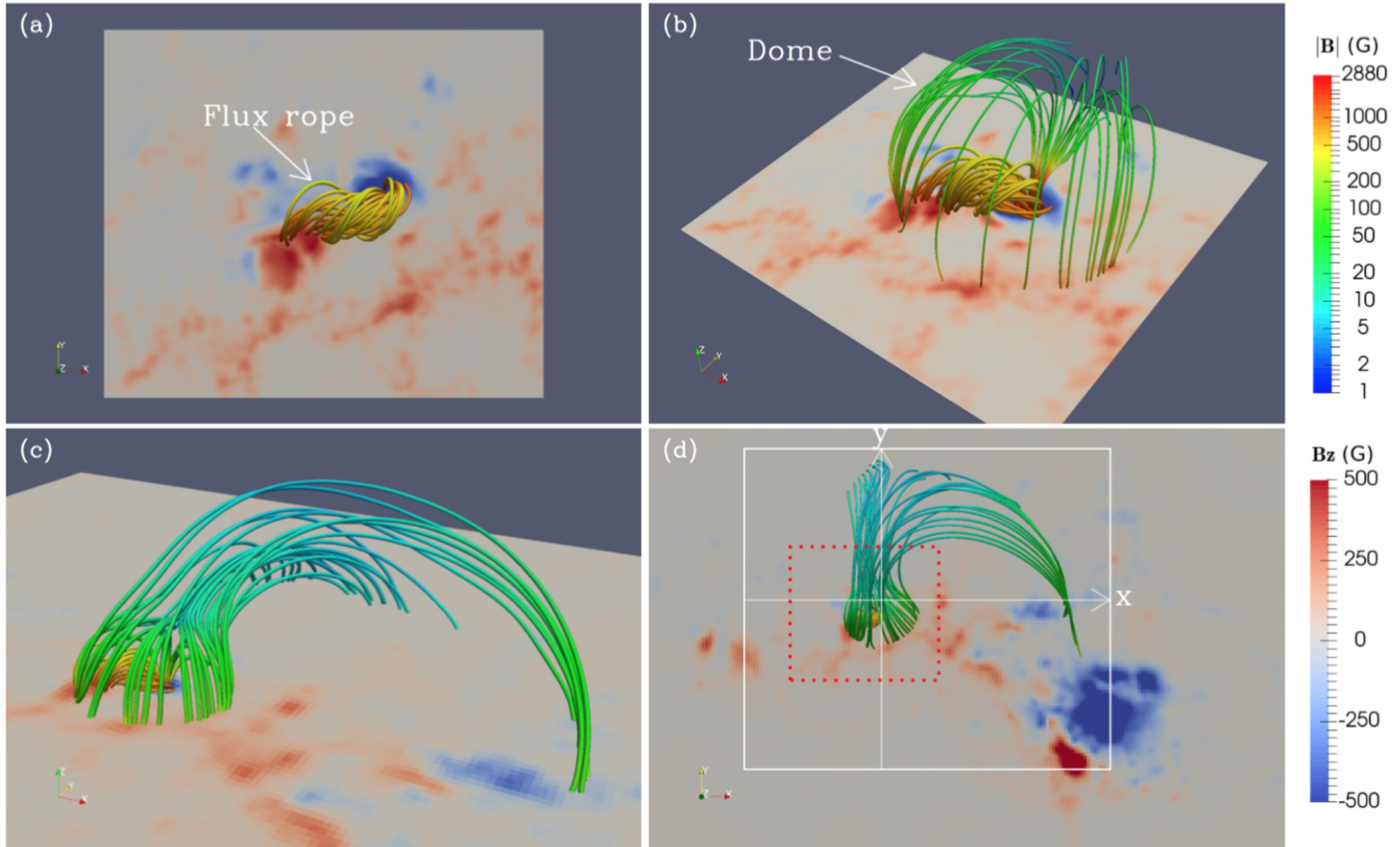
Figure 6. from Observations of a White-light Flare Associated with a Filament Eruption null 2018 APJ 854 64 doi:10.3847/1538-4357/aaa7f1 https://dx.doi.org/10.3847/1538-4357/aaa7f1 © 2018. The American Astronomical Society. All rights reserved.
