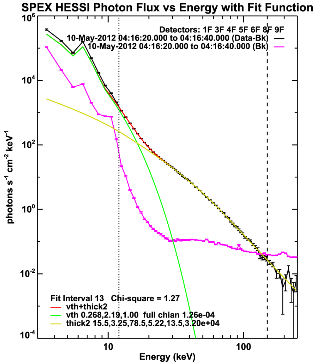
Figure 4. from Observations of a White-light Flare Associated with a Filament Eruption null 2018 APJ 854 64 doi:10.3847/1538-4357/aaa7f1 https://dx.doi.org/10.3847/1538-4357/aaa7f1
