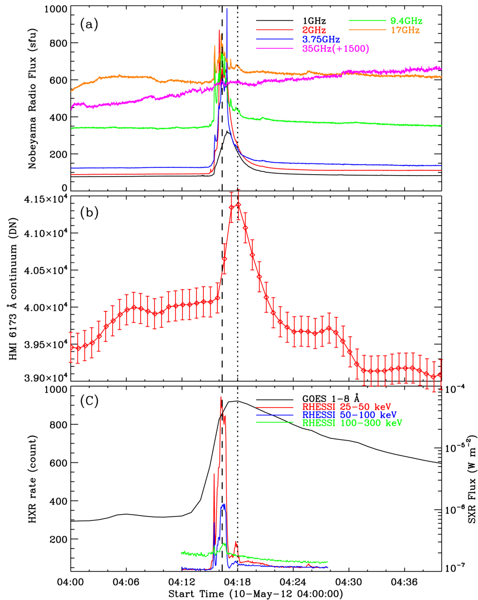
Figure 3. from Observations of a White-light Flare Associated with a Filament Eruption null 2018 APJ 854 64 doi:10.3847/1538-4357/aaa7f1 https://dx.doi.org/10.3847/1538-4357/aaa7f1
