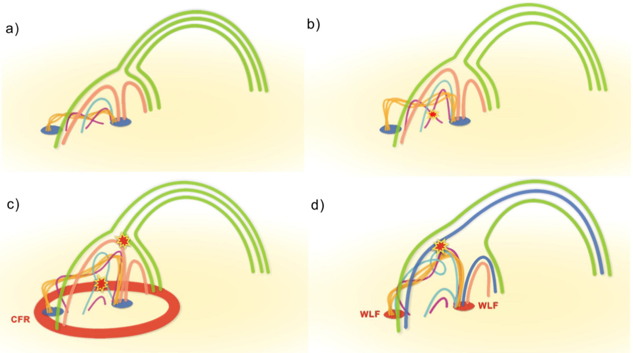
Figure 10. from Observations of a White-light Flare Associated with a Filament Eruption null 2018 APJ 854 64 doi:10.3847/1538-4357/aaa7f1 https://dx.doi.org/10.3847/1538-4357/aaa7f1 © 2018. The American Astronomical Society. All rights reserved.
