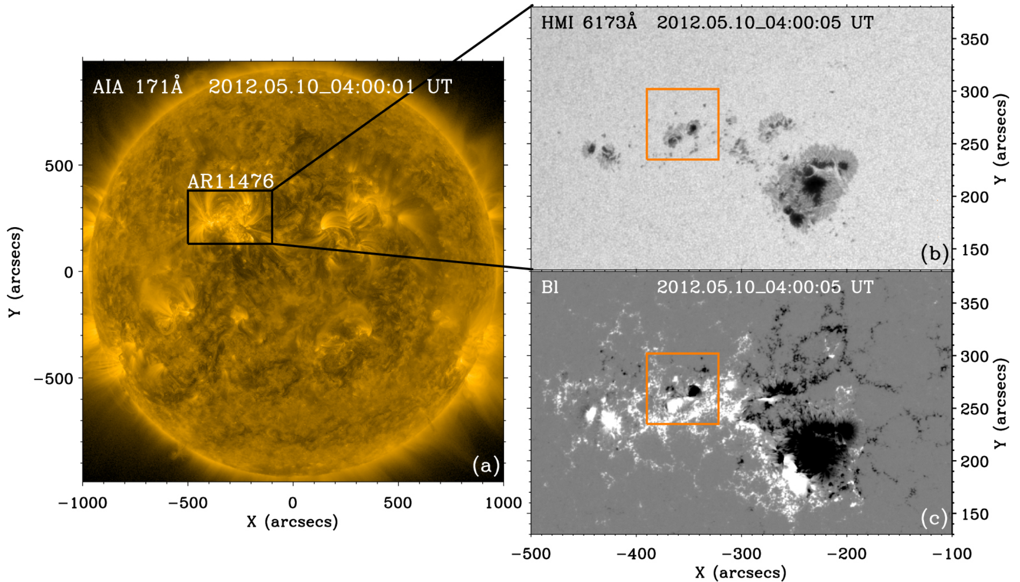
Figure 1. from Observations of a White-light Flare Associated with a Filament Eruption null 2018 APJ 854 64 doi:10.3847/1538-4357/aaa7f1 https://dx.doi.org/10.3847/1538-4357/aaa7f1 © 2018. The American Astronomical Society. All rights reserved.
