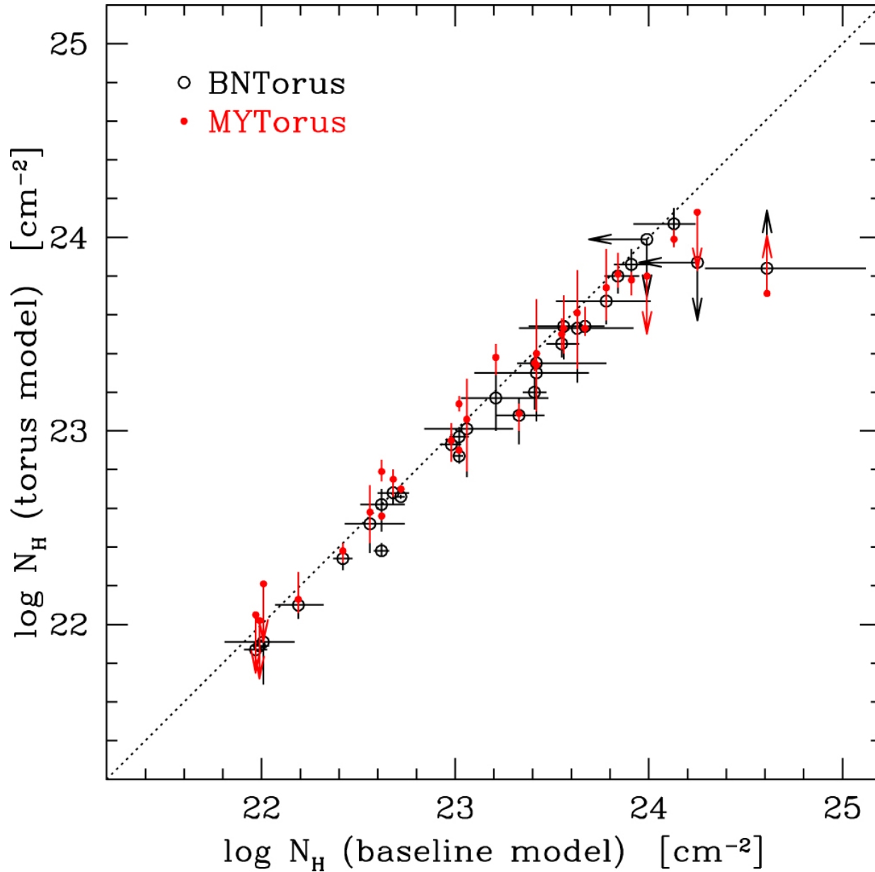
Figure 9. from The NuSTAR Extragalactic Surveys: X-Ray Spectroscopic Analysis of the Bright Hard-band Selected Sample null 2018 APJ 854 33 doi:10.3847/1538-4357/aaa550 https://dx.doi.org/10.3847/1538-4357/aaa550 © 2018. The American Astronomical Society. All rights reserved.
