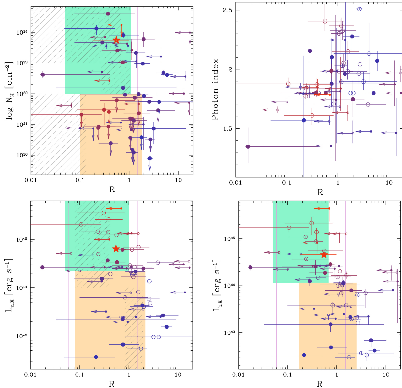
Figure 8. from The NuSTAR Extragalactic Surveys: X-Ray Spectroscopic Analysis of the Bright Hard-band Selected Sample null 2018 APJ 854 33 doi:10.3847/1538-4357/aaa550 https://dx.doi.org/10.3847/1538-4357/aaa550 © 2018. The American Astronomical Society. All rights reserved.
