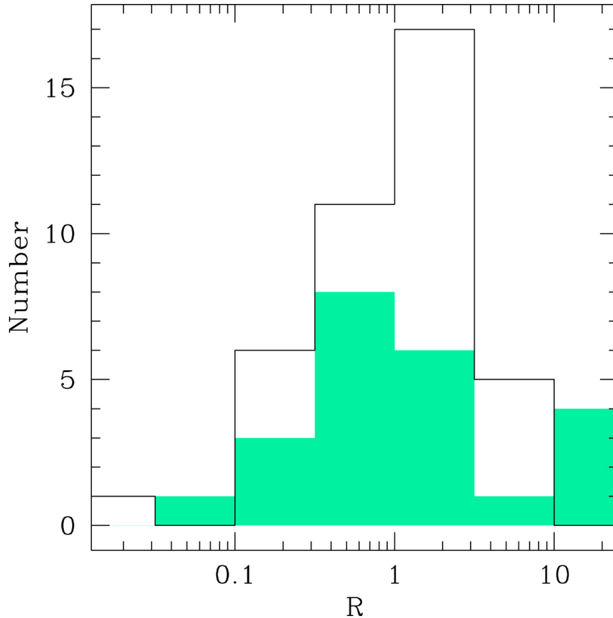
Figure 7. from The NuSTAR Extragalactic Surveys: X-Ray Spectroscopic Analysis of the Bright Hard-band Selected Sample null 2018 APJ 854 33 doi:10.3847/1538-4357/aaa550 https://dx.doi.org/10.3847/1538-4357/aaa550 © 2018. The American Astronomical Society. All rights reserved.
